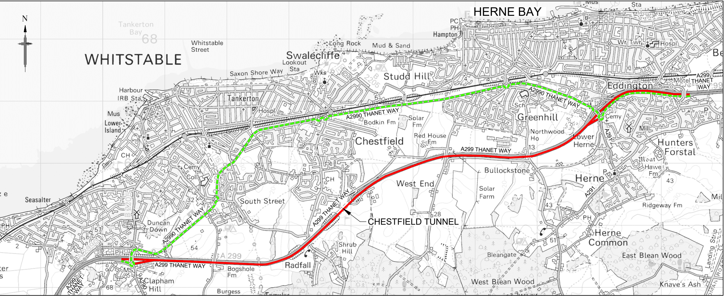
DIVERSION FOR WESTBOUND CLOSURE - OVERVIEW PLAN
