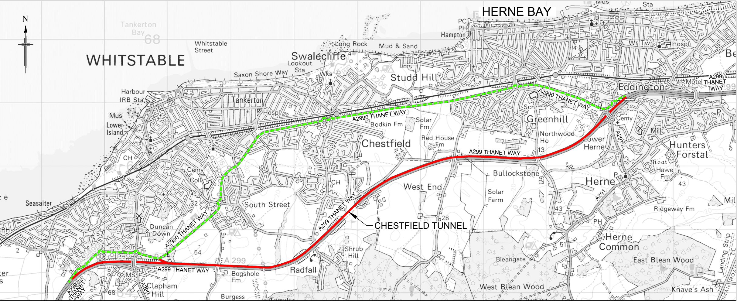
DIVERSION FOR EASTBOUND CLOSURE - OVERVIEW PLAN
