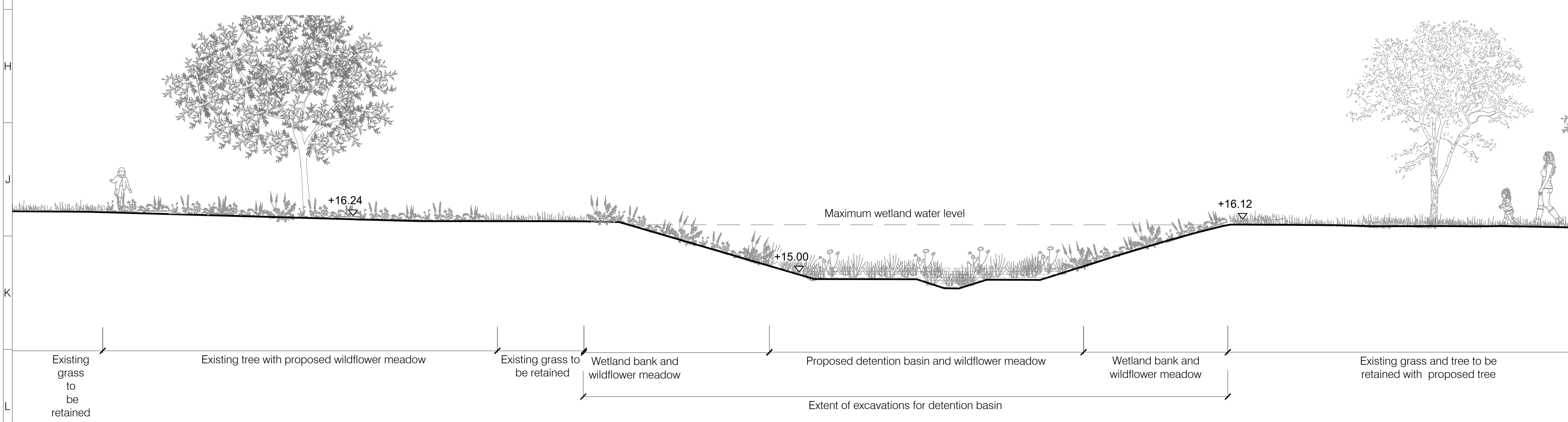
03 WETLAND BASIN CROSS SECTION 3003-01 SECTION
