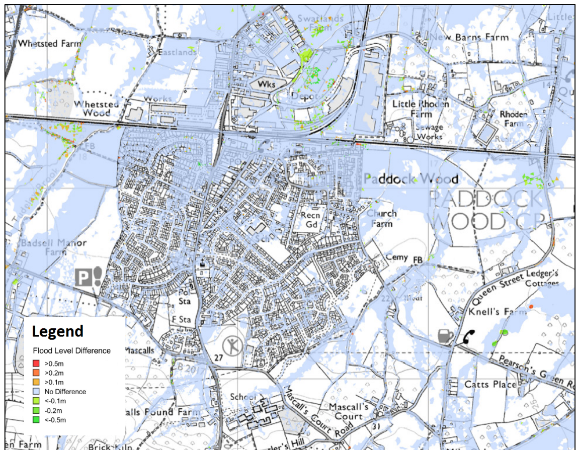
Figure 3-2 The Difference in flood extent for the 1 in 100 event for the Rhoden culvert capacity as is and the Rhoden culvert capacity doubled
