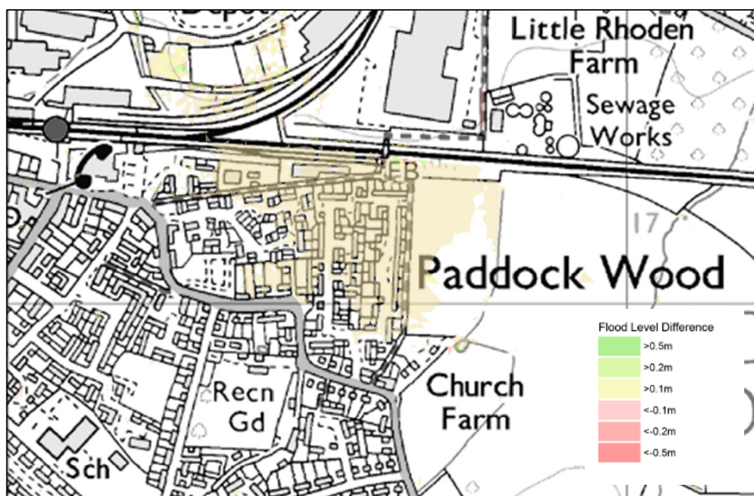
Figure 3-4 The Difference in flood depth for the 1 in 100 event for the Rhoden culvert capacity as is and the Rhoden culvert capacity doubled
