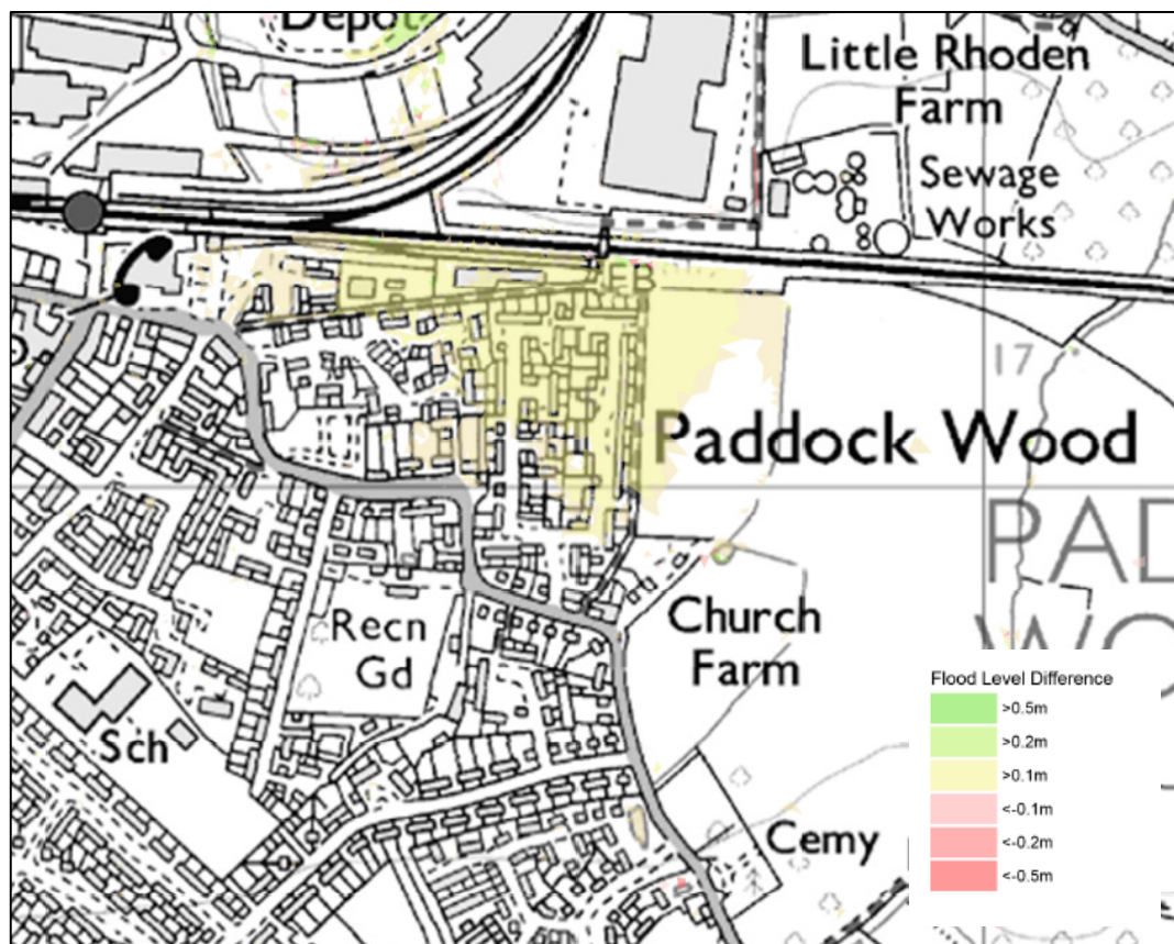
Figure 3-3 The Difference in flood depth for the 1 in 50 event for the Rhoden culvert capacity as is and the Rhoden culvert capacity doubled
